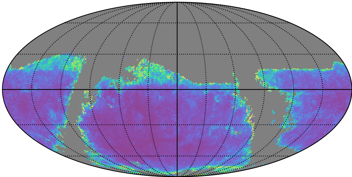
too_combined_s1.0_split_v3.4_10yrs g band: AGN SF_uncert
