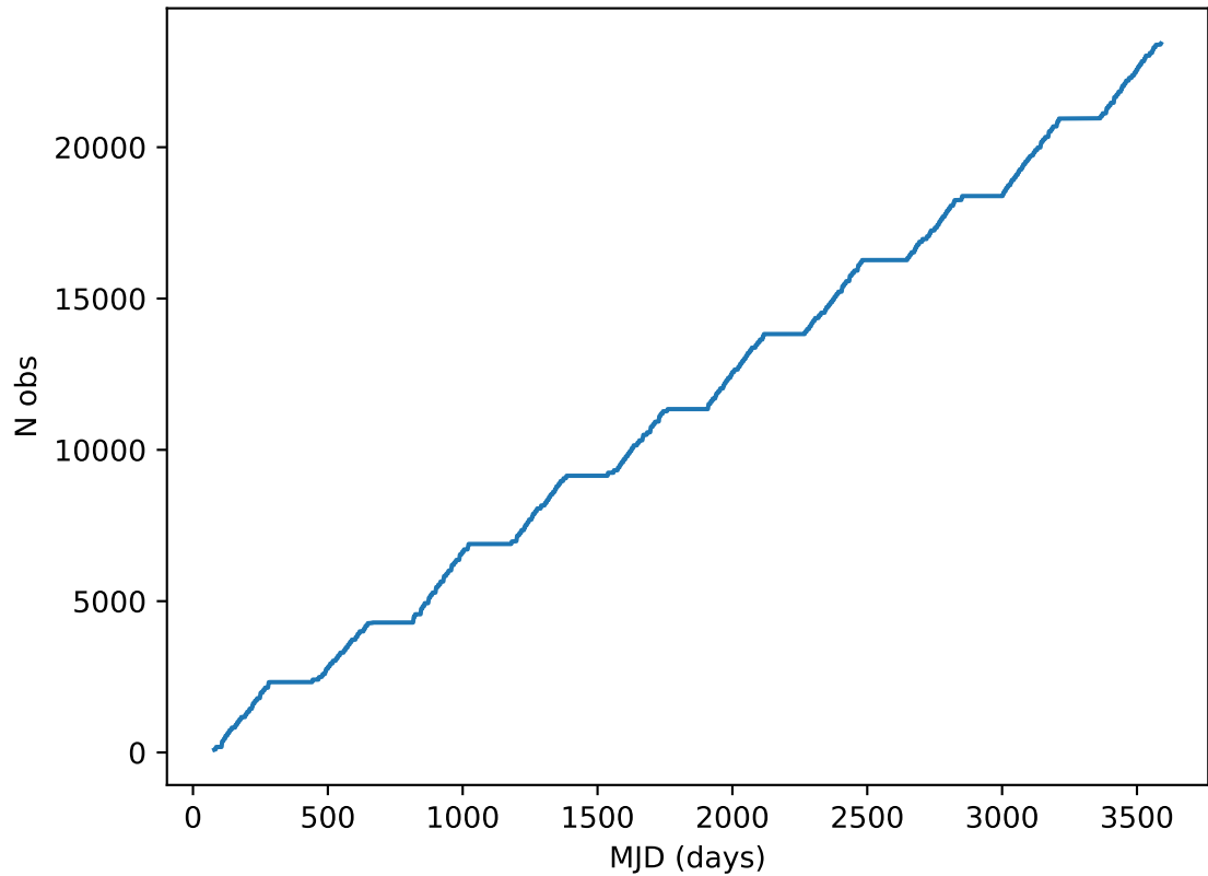
too_combined_s1.0_split_v3.4_10yrs all bands: DD:XMM_LSS Cumulative NVisits
