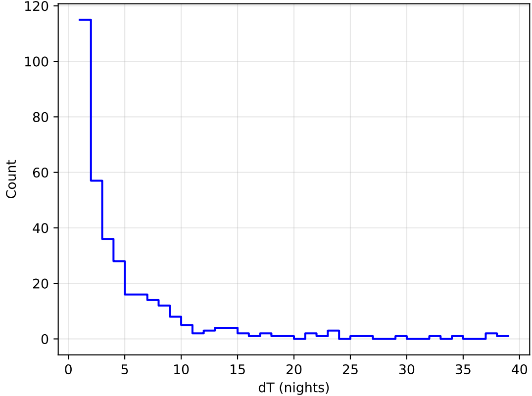
too_combined_s1.0_split_v3.4_10yrs all bands: DD:WFD Delta Nights Histogram
