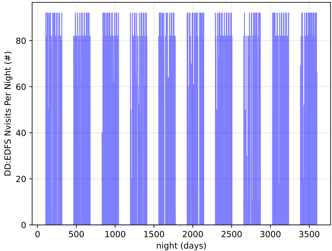
too_combined_s1.0_split_v3.4_10yrs all bands: DD:EDFS Nvisits Per Night
