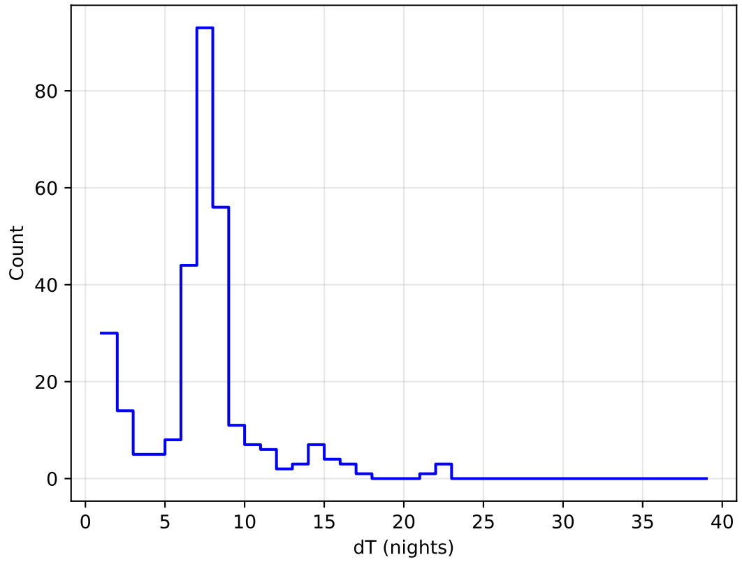
too_combined_s1.0_split_v3.4_10yrs all bands: DD:EDFS Delta Nights Histogram
