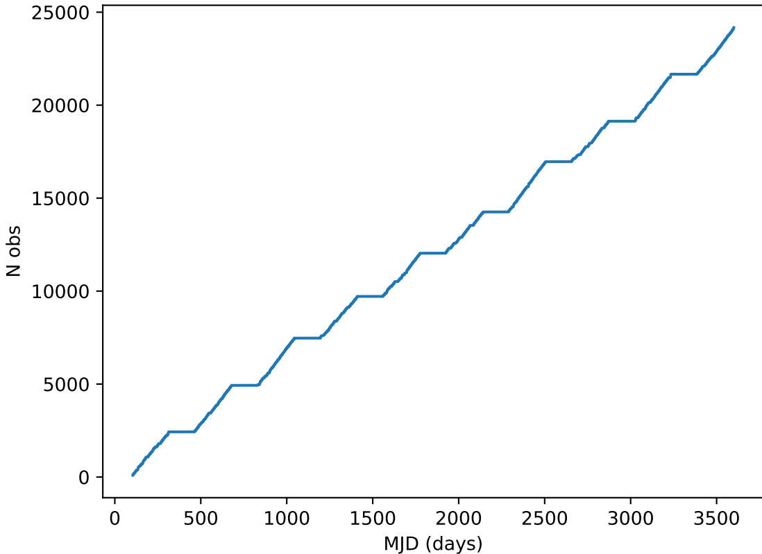
too_combined_s1.0_split_v3.4_10yrs all bands: DD:EDFS Cumulative NVisits
