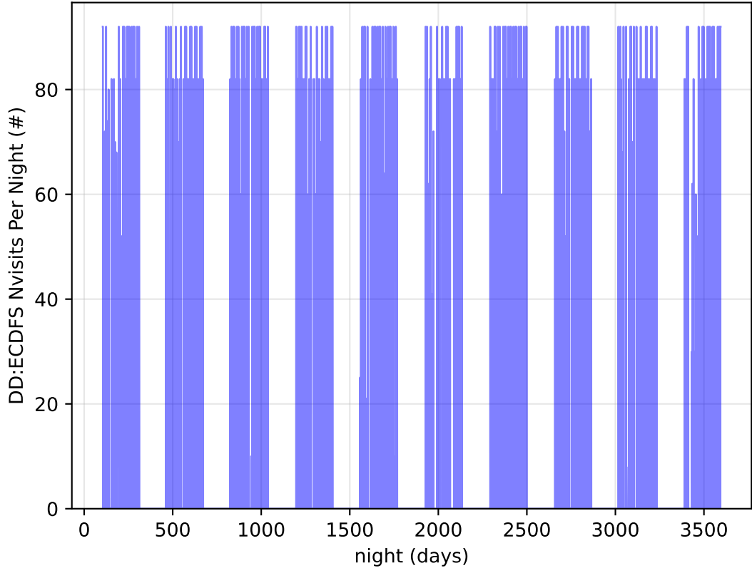
too_combined_s1.0_split_v3.4_10yrs all bands: DD:ECDFS Nvisits Per Night
