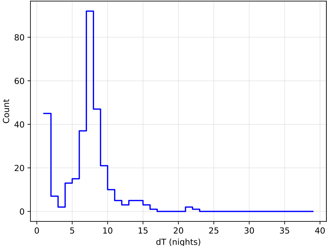
too_combined_s1.0_split_v3.4_10yrs all bands: DD:ECDFS Delta Nights Histogram
