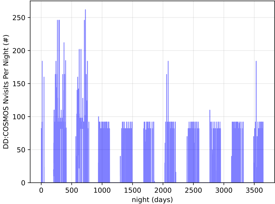
too_combined_s1.0_split_v3.4_10yrs all bands: DD: COSMOS Nvisits Per Night
