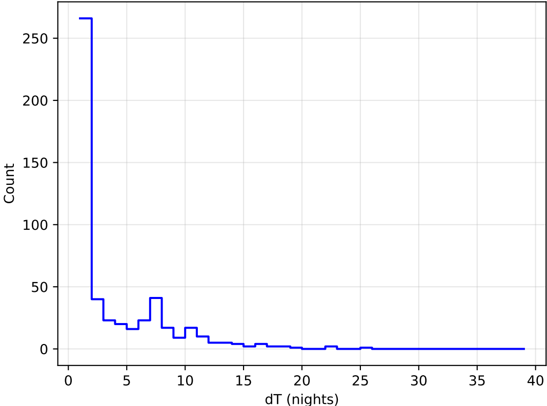
too_combined_s1.0_split_v3.4_10yrs all bands: DD: COSMOS Delta Nights Histogram
