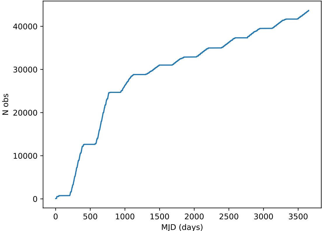
too_combined_s1.0_split_v3.4_10yrs all bands: DD: COSMOS Cumulative NVisits
