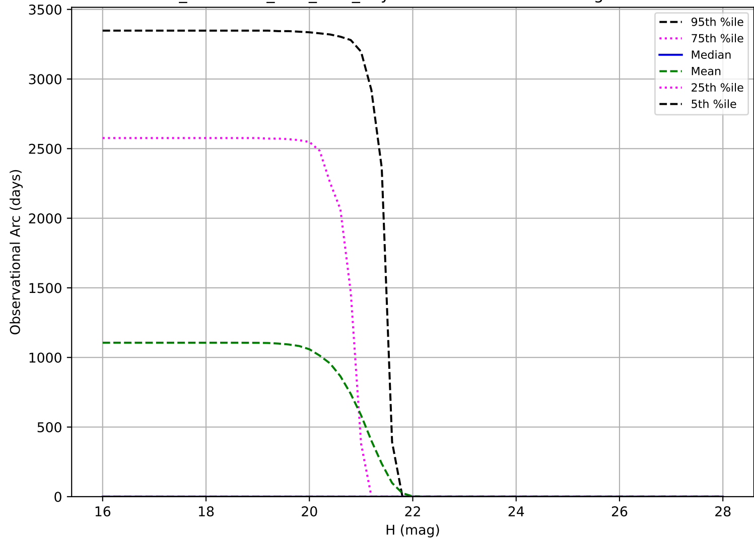
too_combined_s0.8_v3.4_10yrs: Observational Arc Length Vatra
