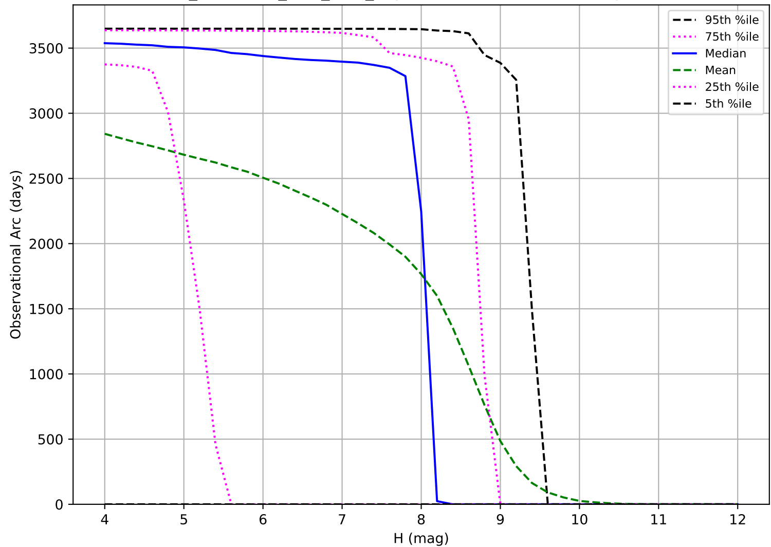
too_combined_s0.8_v3.4_10yrs: Observational Arc Length TNO
