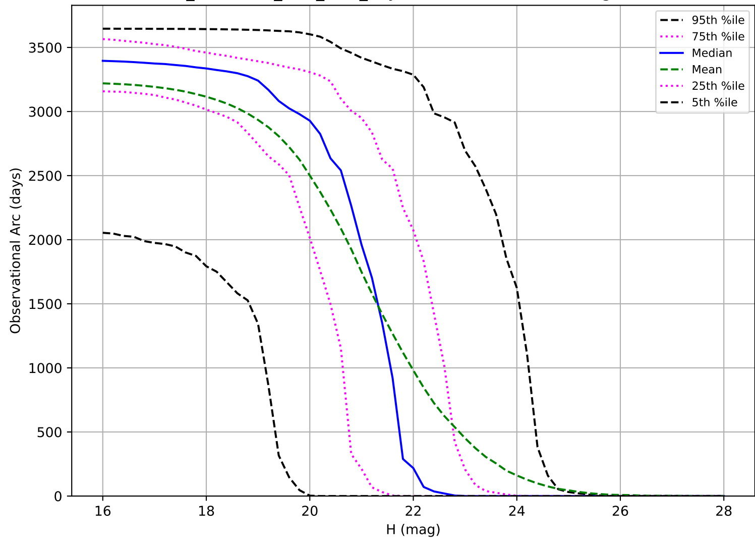
too_combined_s0.8_v3.4_10yrs: Observational Arc Length PHA
