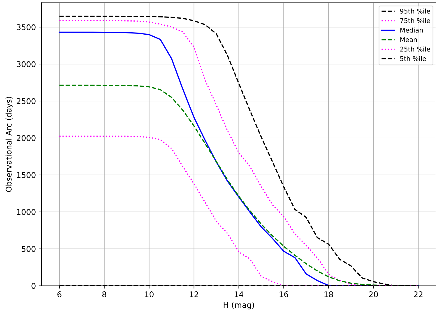
too_combined_s0.8_v3.4_10yrs: Observational Arc Length OCC_r5
