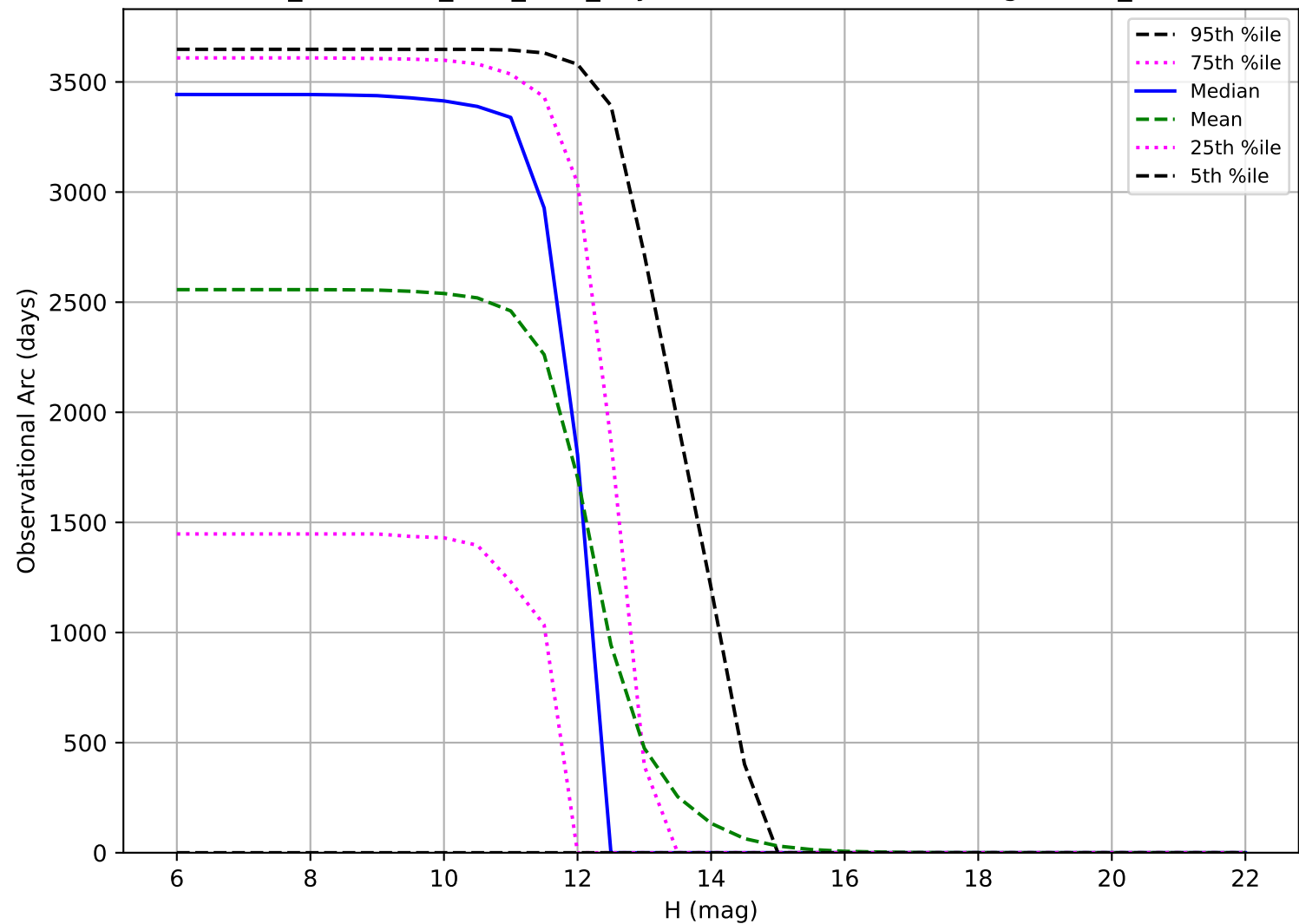
too_combined_s0.8_v3.4_10yrs: Observational Arc Length OCC_r20
