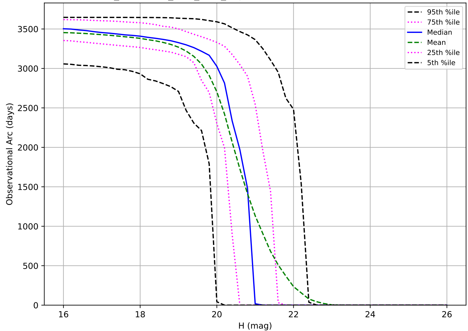
too_combined_s0.8_v3.4_10yrs: Observational Arc Length MBA
