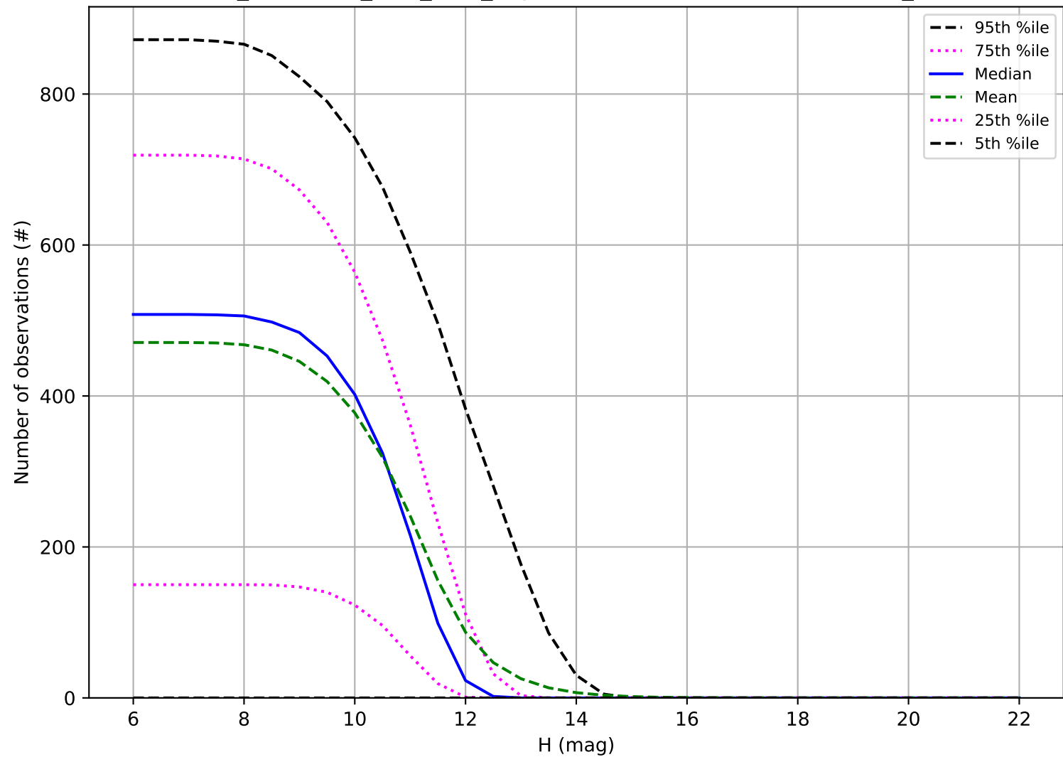
too_combined_s0.8_v3.4_10yrs: Number of observations OCC_r20
