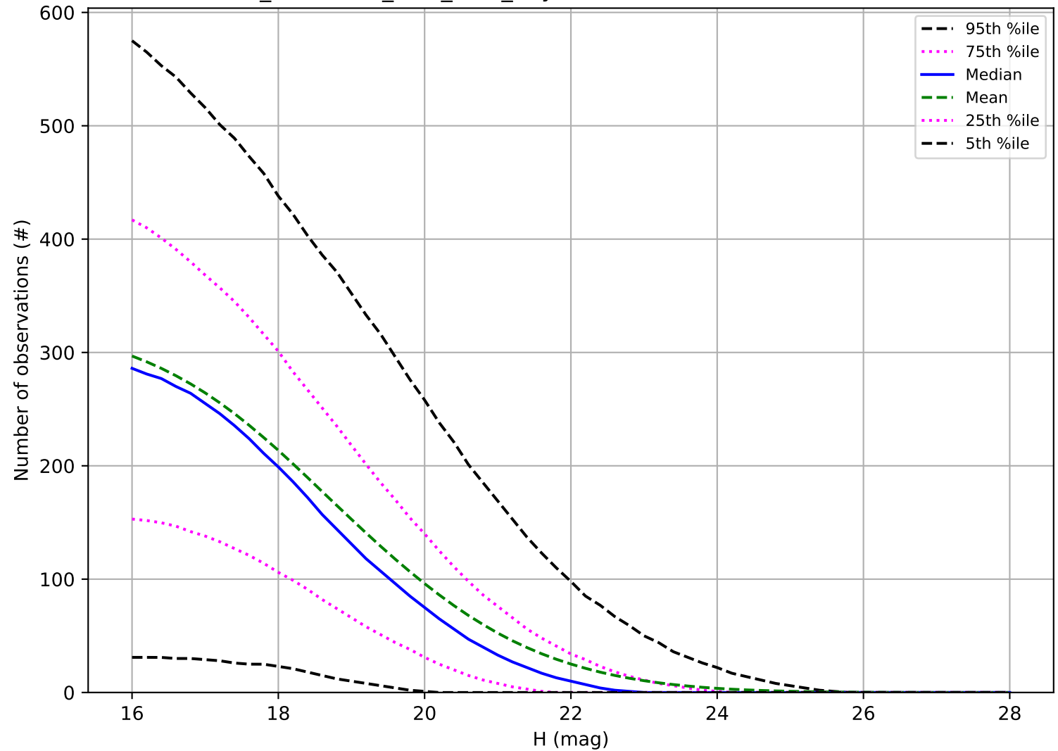
too_combined_s0.8_v3.4_10yrs: Number of observations NEO
