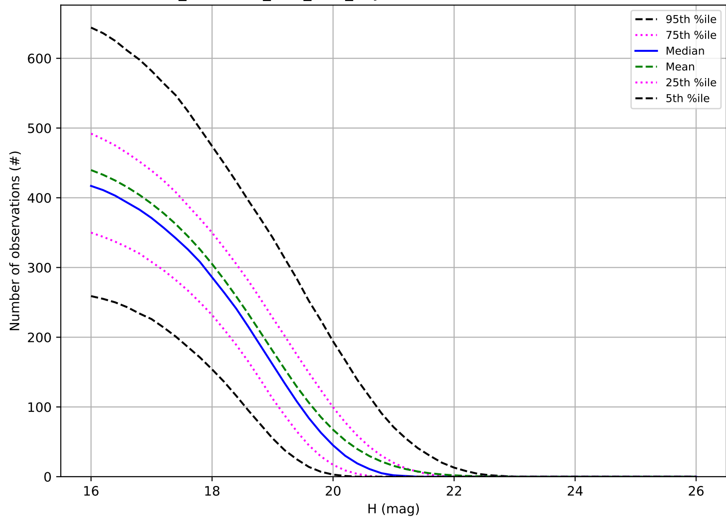
too_combined_s0.8_v3.4_10yrs: Number of observations MBA
