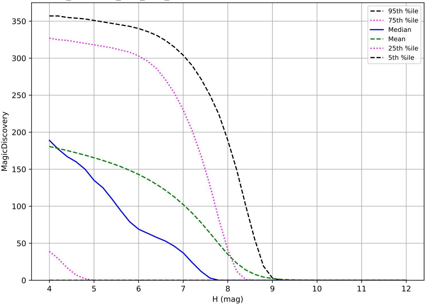
too_combined_s0.8_v3.4_10yrs: TNO 6 detections in 60 nights detection loss
