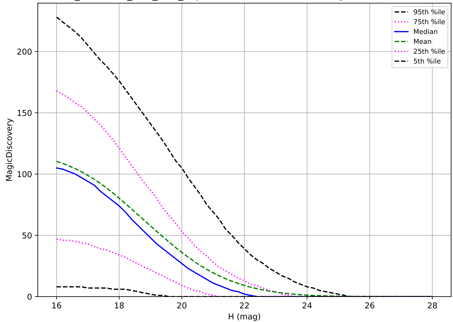
too_combined_s0.8_v3.4_10yrs: PHA 6 detections in 60 nights detection loss
