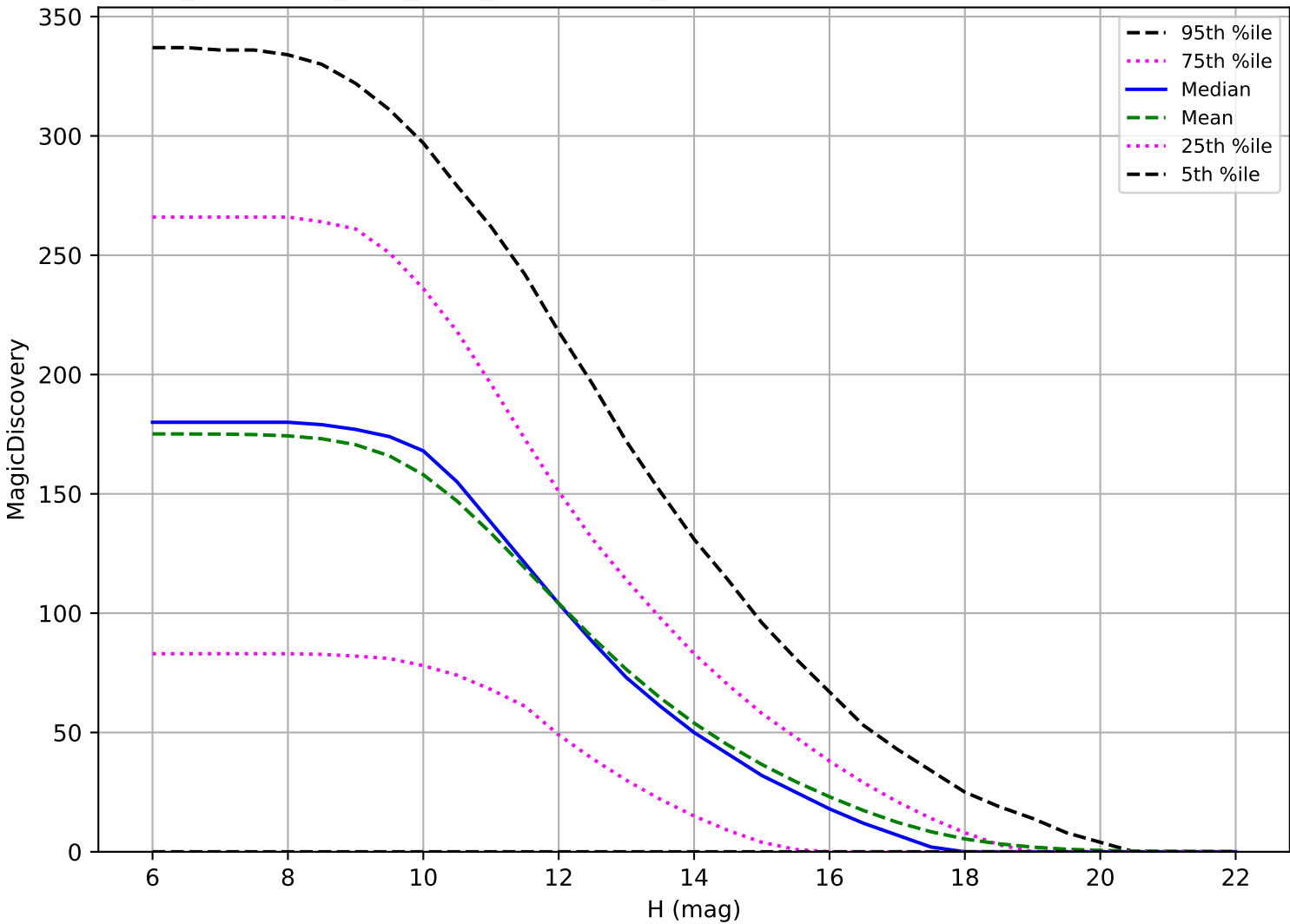
too_combined_s0.8_v3.4_10yrs: OCC_r5 6 detections in 60 nights detection loss
