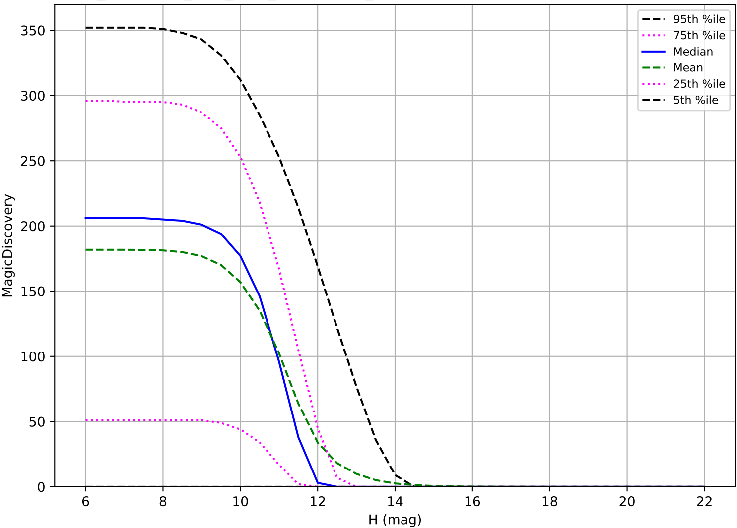
too_combined_s0.8_v3.4_10yrs: OCC_r20 6 detections in 60 nights detection loss
