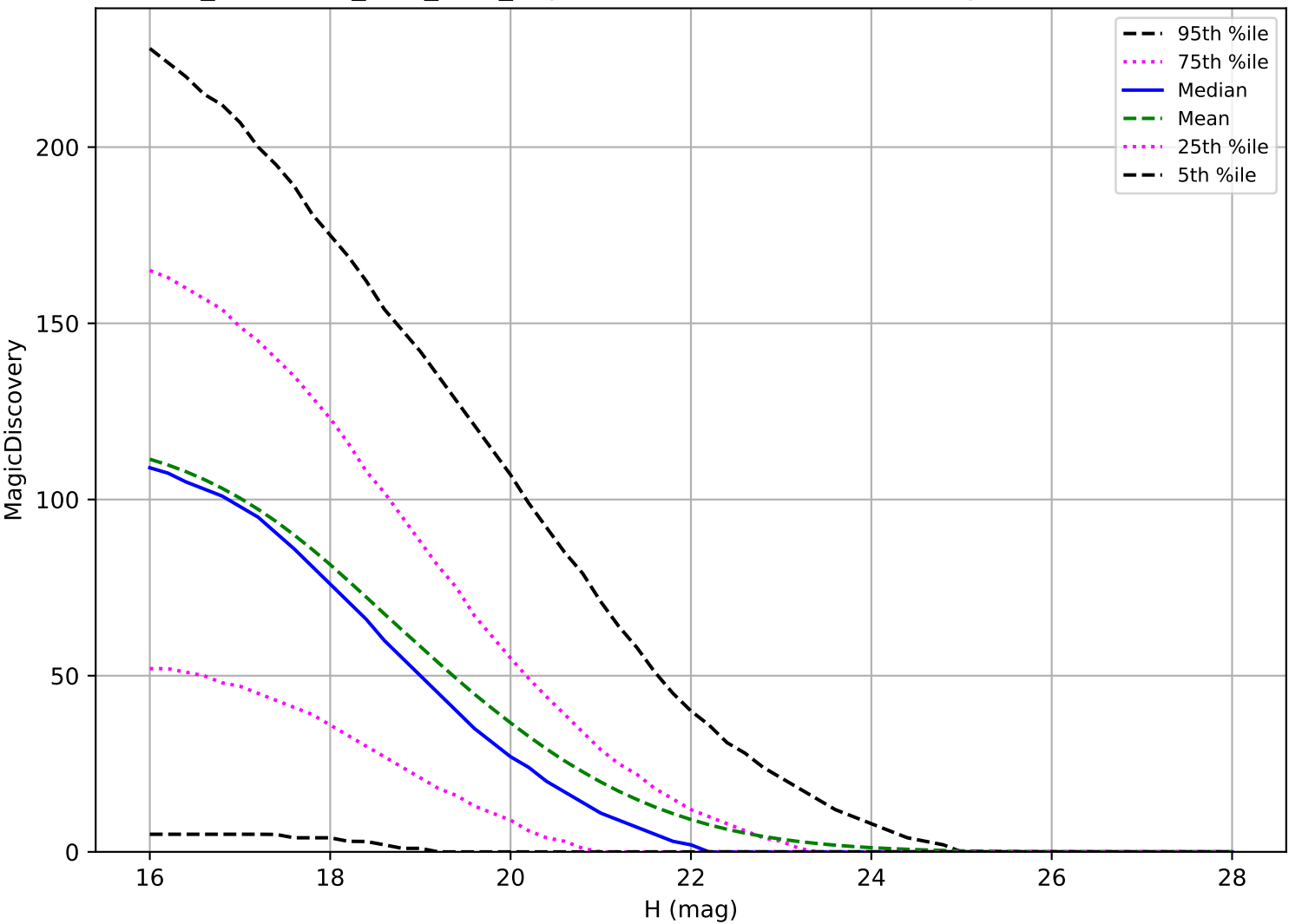
too_combined_s0.8_v3.4_10yrs: NEO 6 detections in 60 nights detection loss
