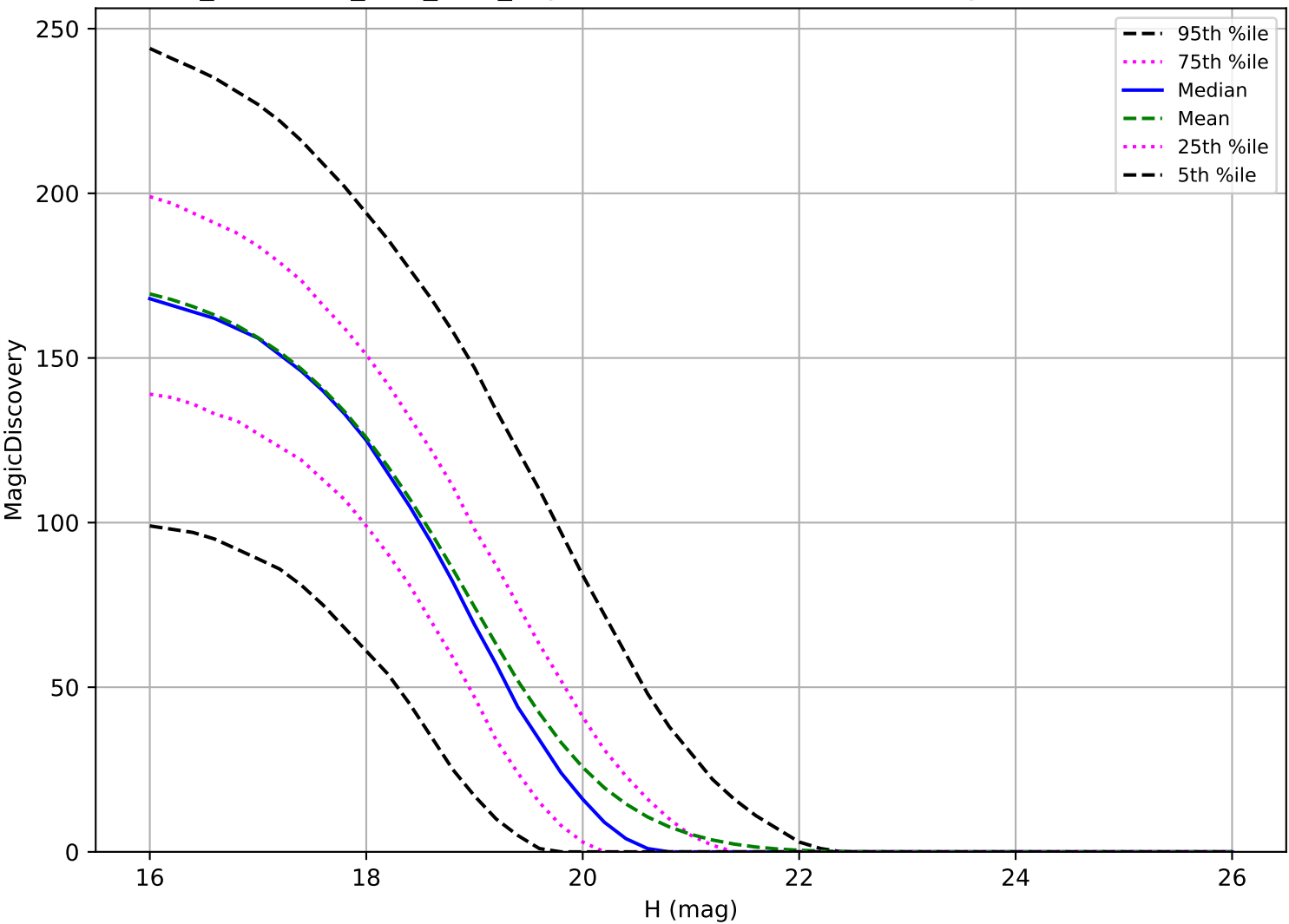
too_combined_s0.8_v3.4_10yrs: MBA 6 detections in 60 nights detection loss
