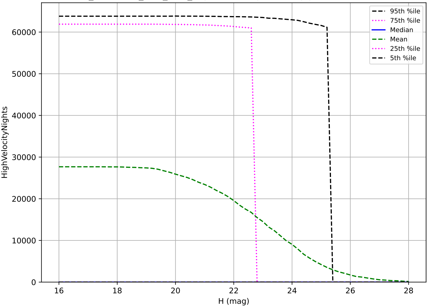
too_combined_s0.8_v3.4_10yrs: PHA High velocity pair detection loss
