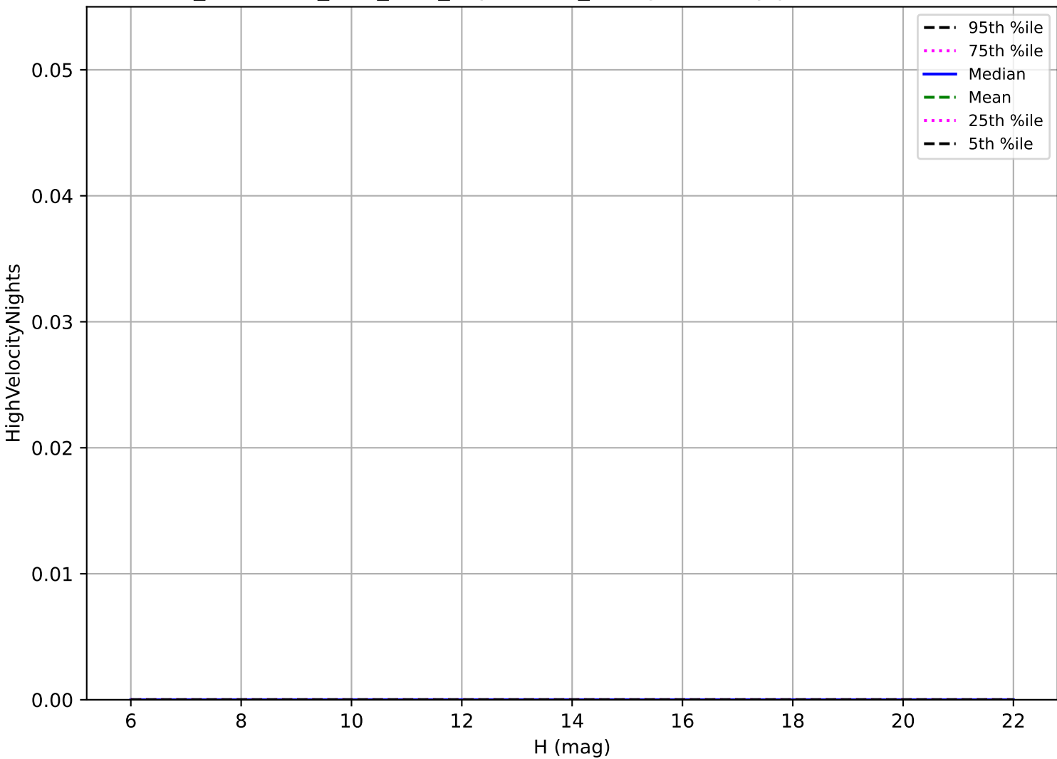
too_combined_s0.8_v3.4_10yrs: OCC_r5 High velocity pair detection loss
