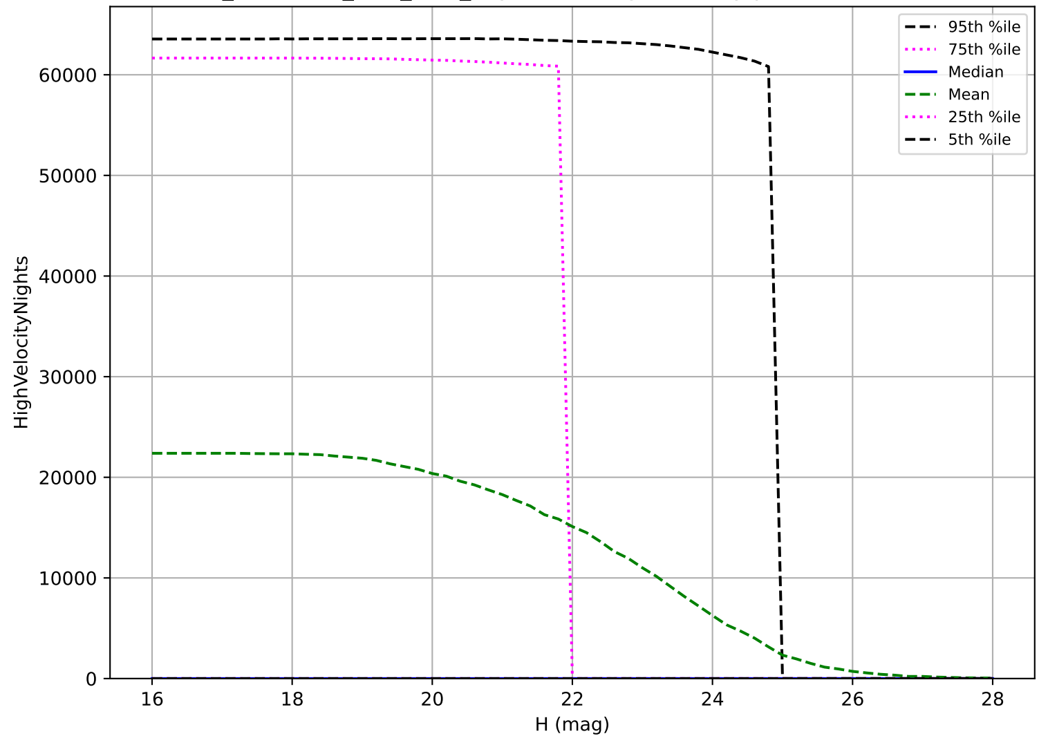
too_combined_s0.8_v3.4_10yrs: NEO High velocity pair detection loss
