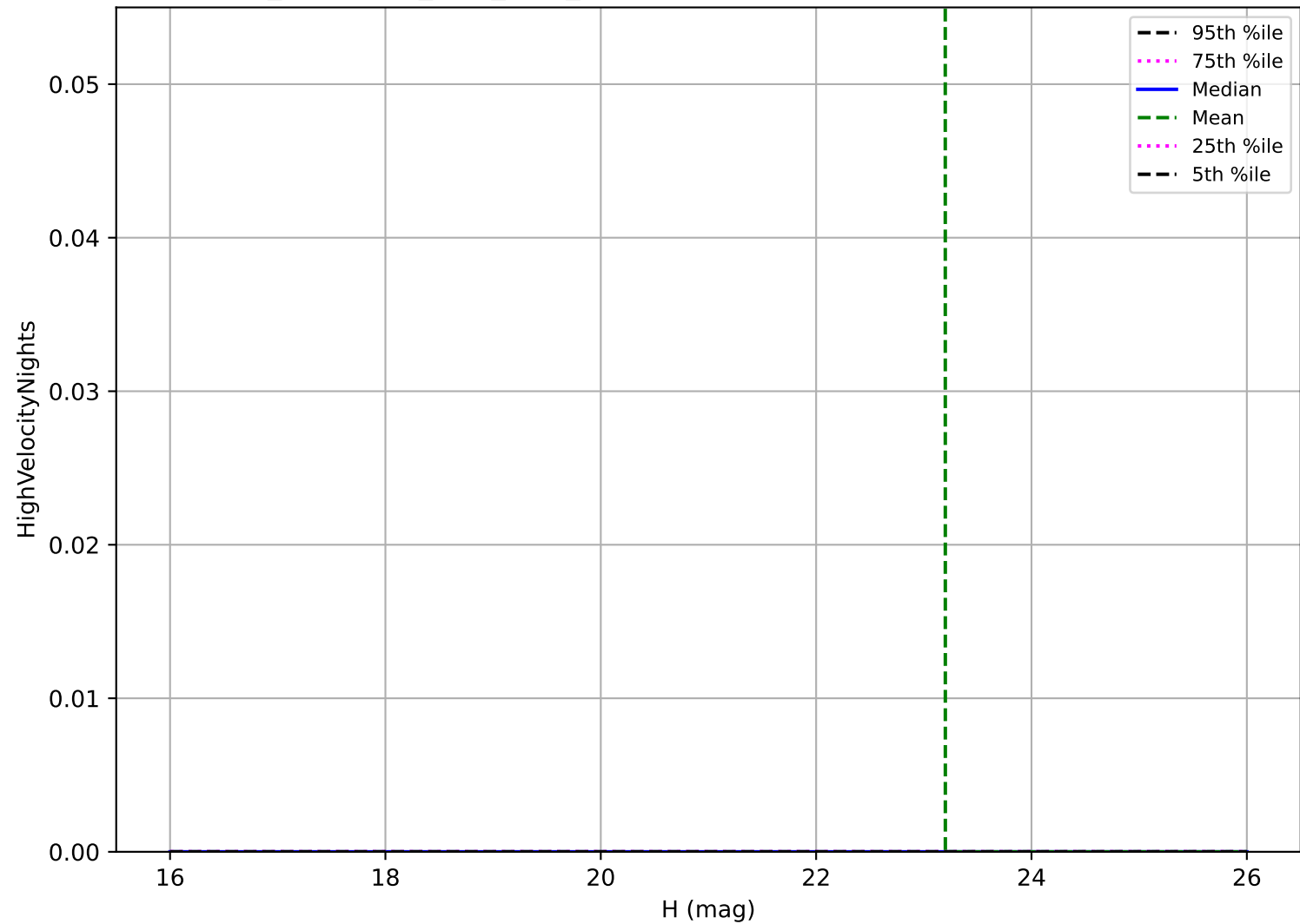
too_combined_s0.8_v3.4_10yrs: MBA High velocity pair detection loss
