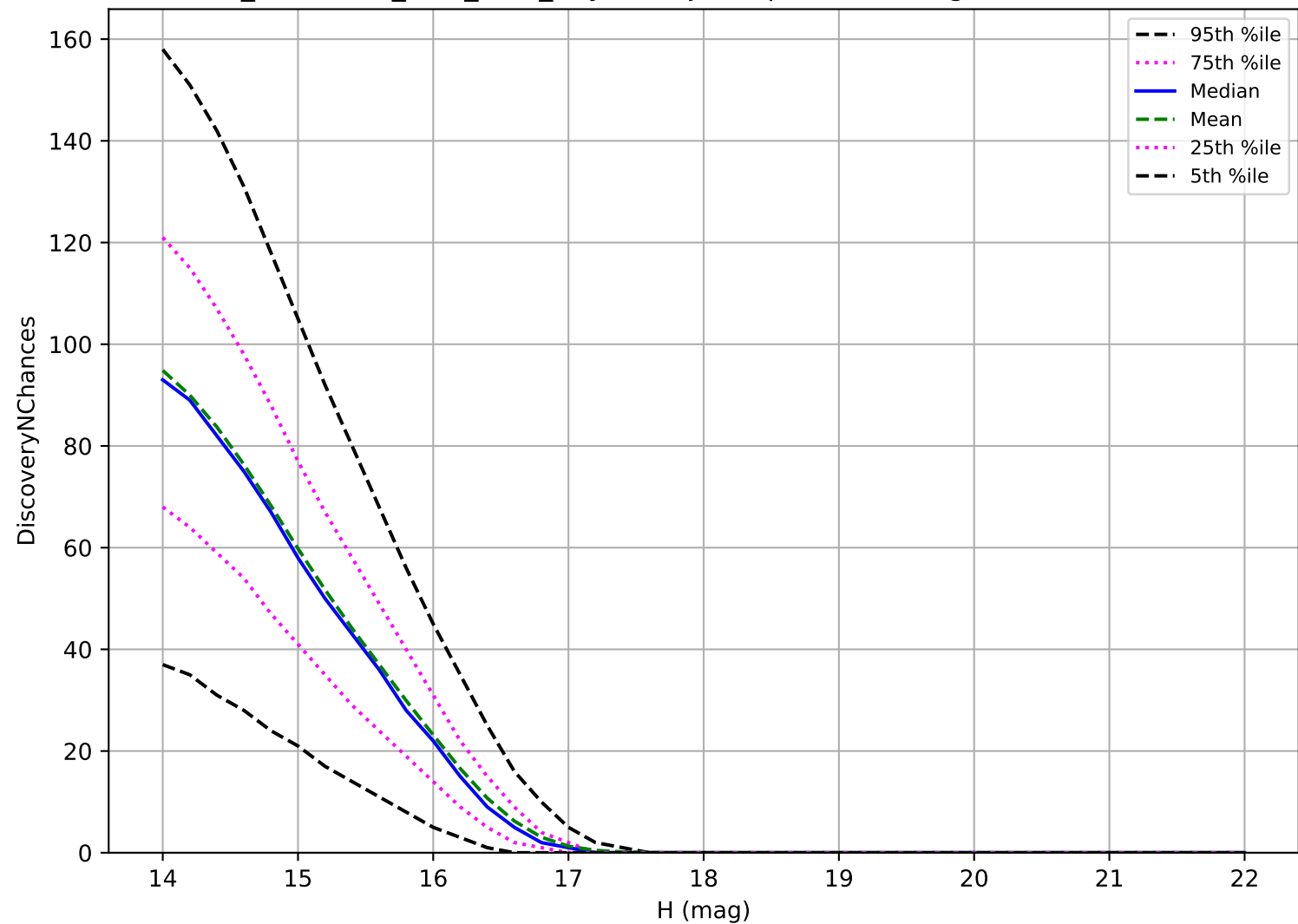
too_combined_s0.8_v3.4_10yrs: Trojan 3 pairs in 15 nights detection loss
