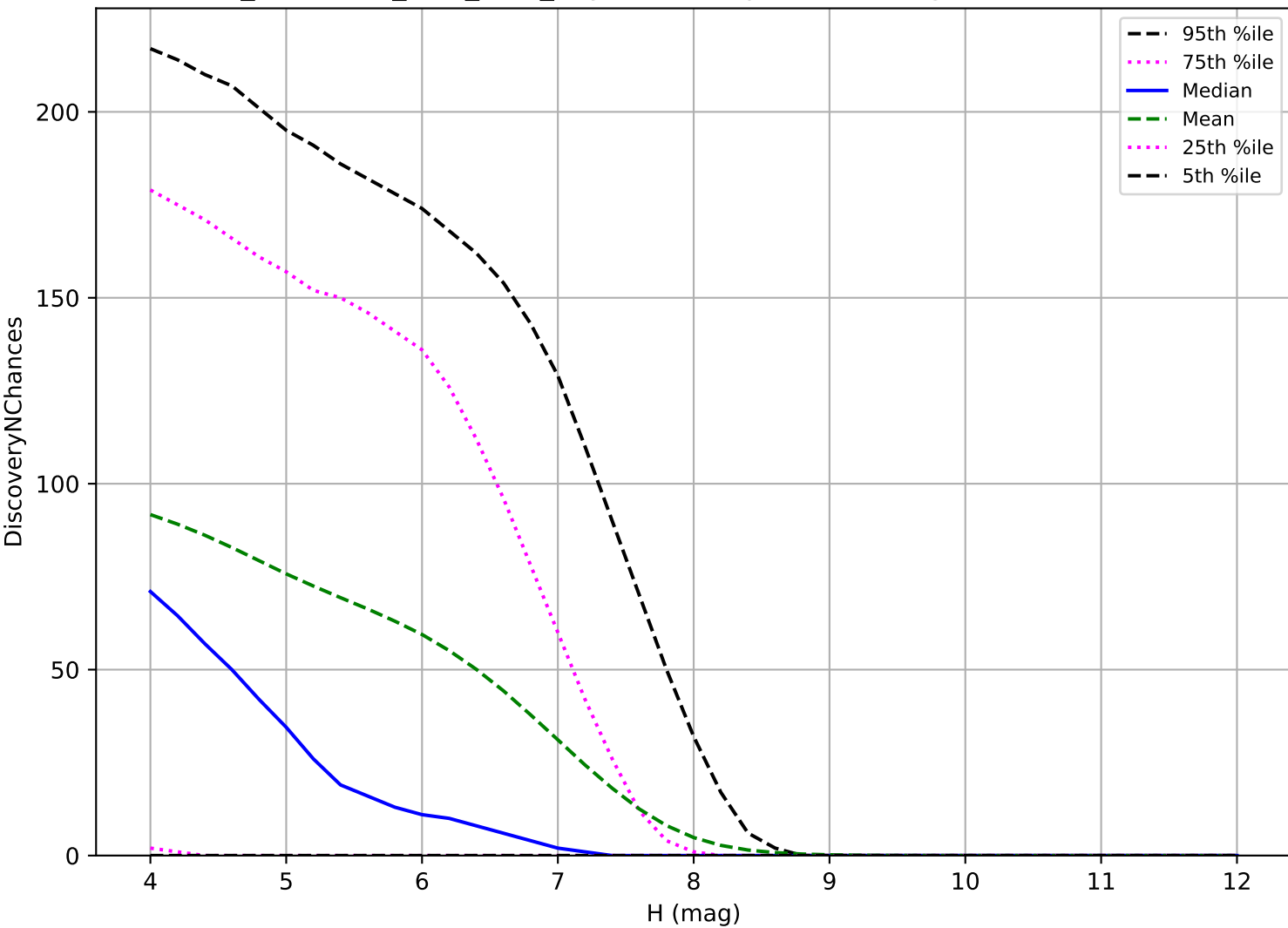
too_combined_s0.8_v3.4_10yrs: TNO 3 pairs in 15 nights detection loss
