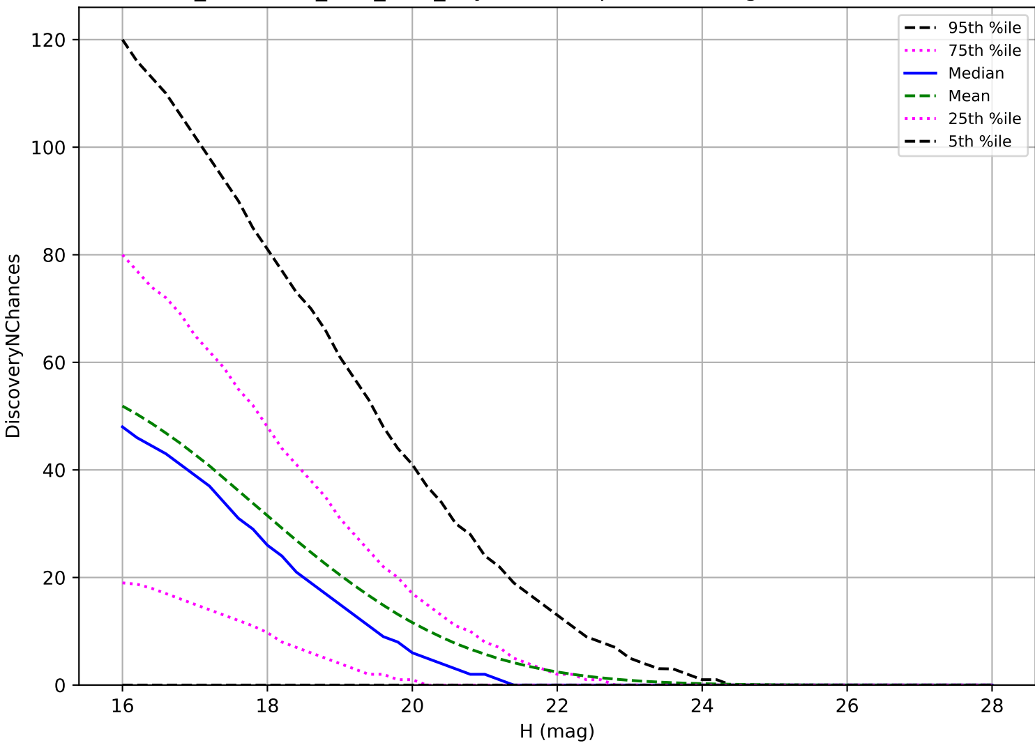
too_combined_s0.8_v3.4_10yrs: NEO 3 pairs in 15 nights detection loss
