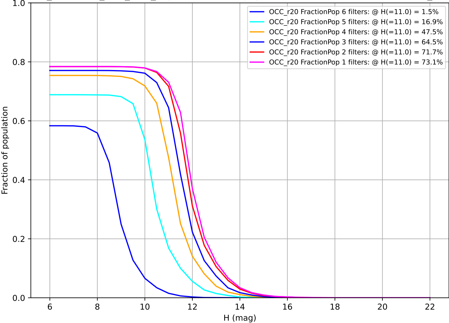
too_combined_s0.8_v3.4_10yrs: Fraction of population with colors in X filters OCC_r20
