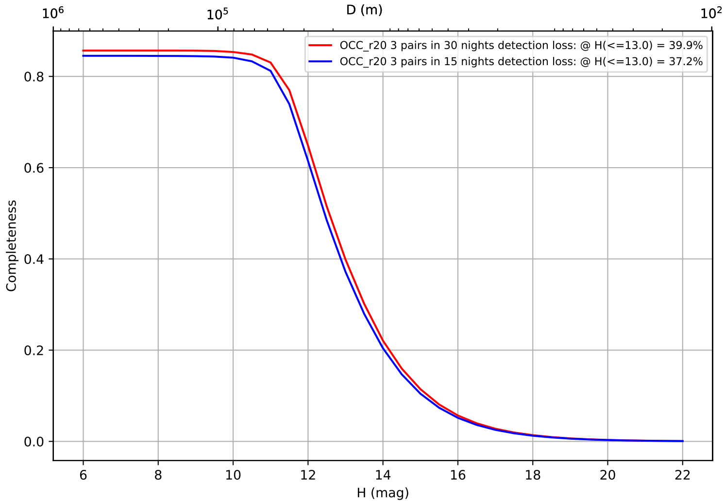
too_combined_s0.8_v3.4_10yrs: CumulativeCompleteness
