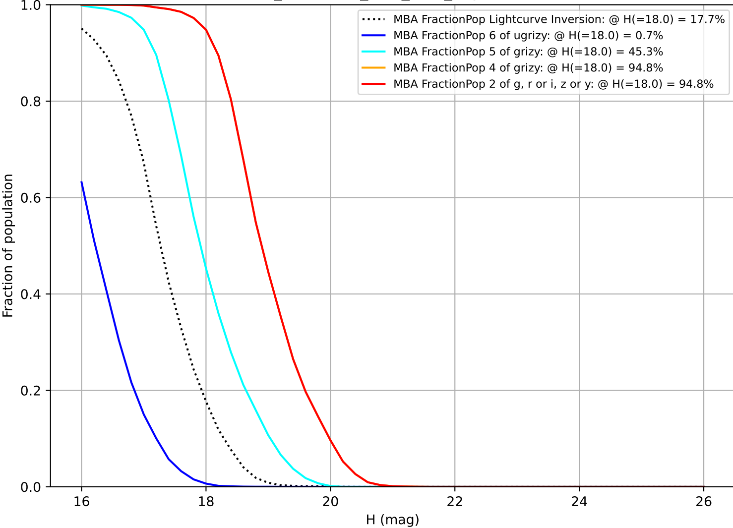
too_combined_s0.8_v3.4_10yrs MBA
