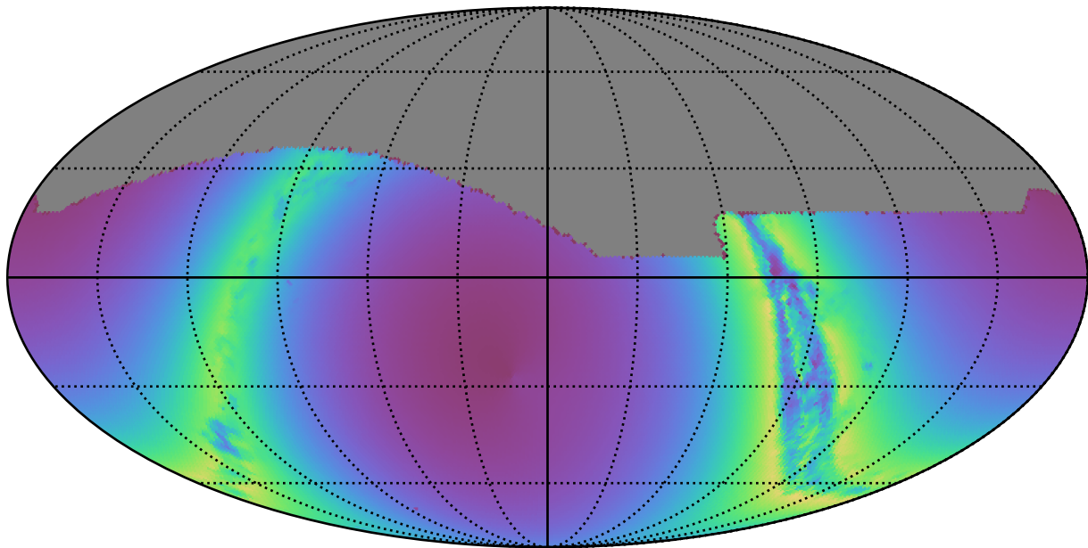
too_combined_s0.8_v3.4_10yrs : young_stars
