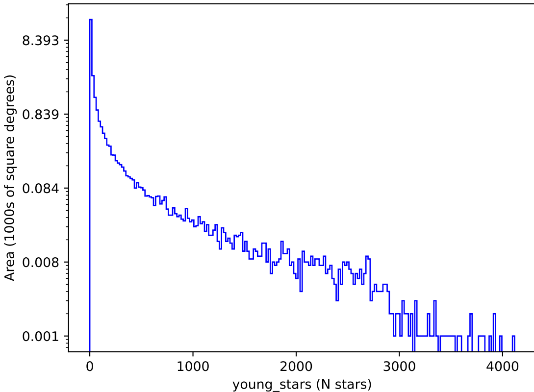
too_combined_s0.8_v3.4_10yrs : young_stars
