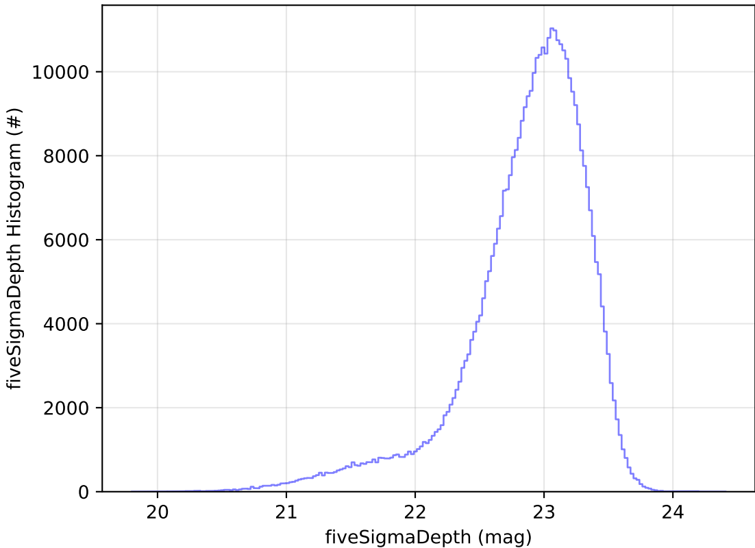
too_combined_s0.8_v3.4_10yrs z: fiveSigmaDepth Histogram
