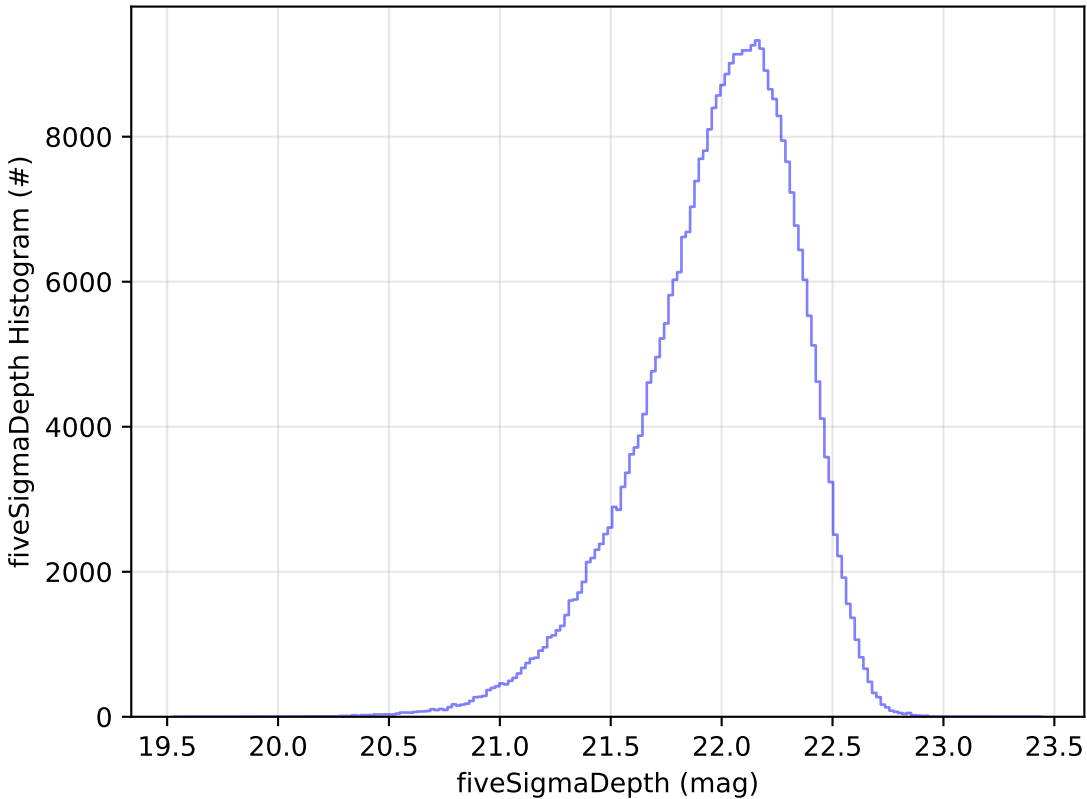
too_combined_s0.8_v3.4_10yrs y: fiveSigmaDepth Histogram
