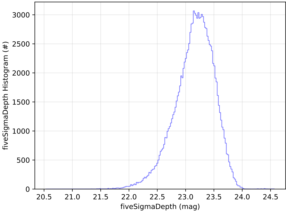
too_combined_s0.8_v3.4_10yrs u: fiveSigmaDepth Histogram
