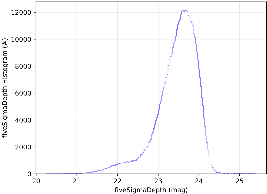
too_combined_s0.8_v3.4_10yrs i: fiveSigmaDepth Histogram
