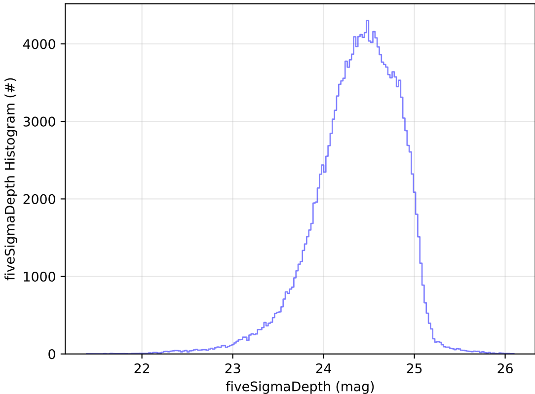
too_combined_s0.8_v3.4_10yrs g: fiveSigmaDepth Histogram
