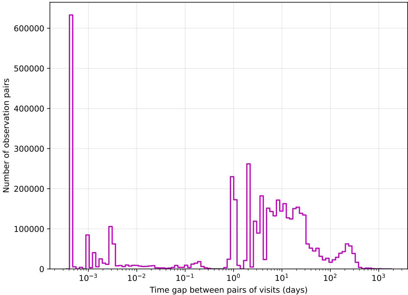
too_combined_s0.8_v3.4_10yrs z band: Tgaps observationStartMJD
