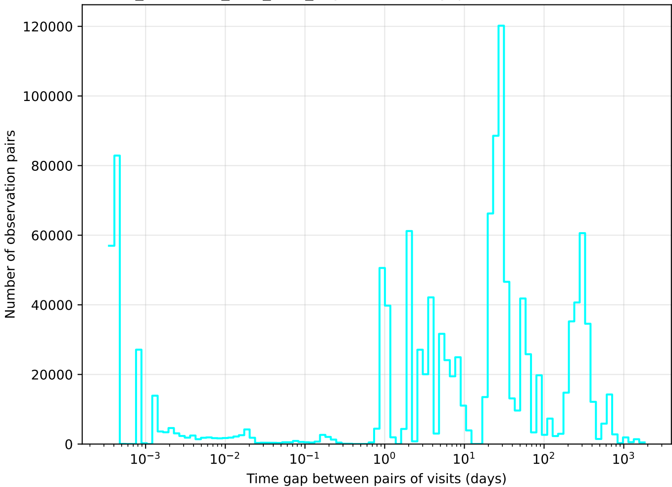
too_combined_s0.8_v3.4_10yrs u band: Tgaps observationStartMJD
