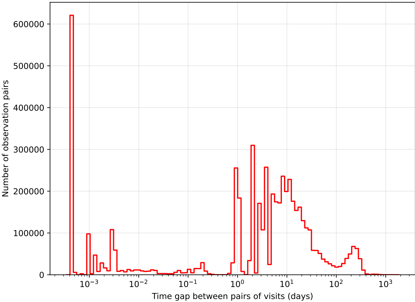
too_combined_s0.8_v3.4_10yrs i band: Tgaps observationStartMJD
