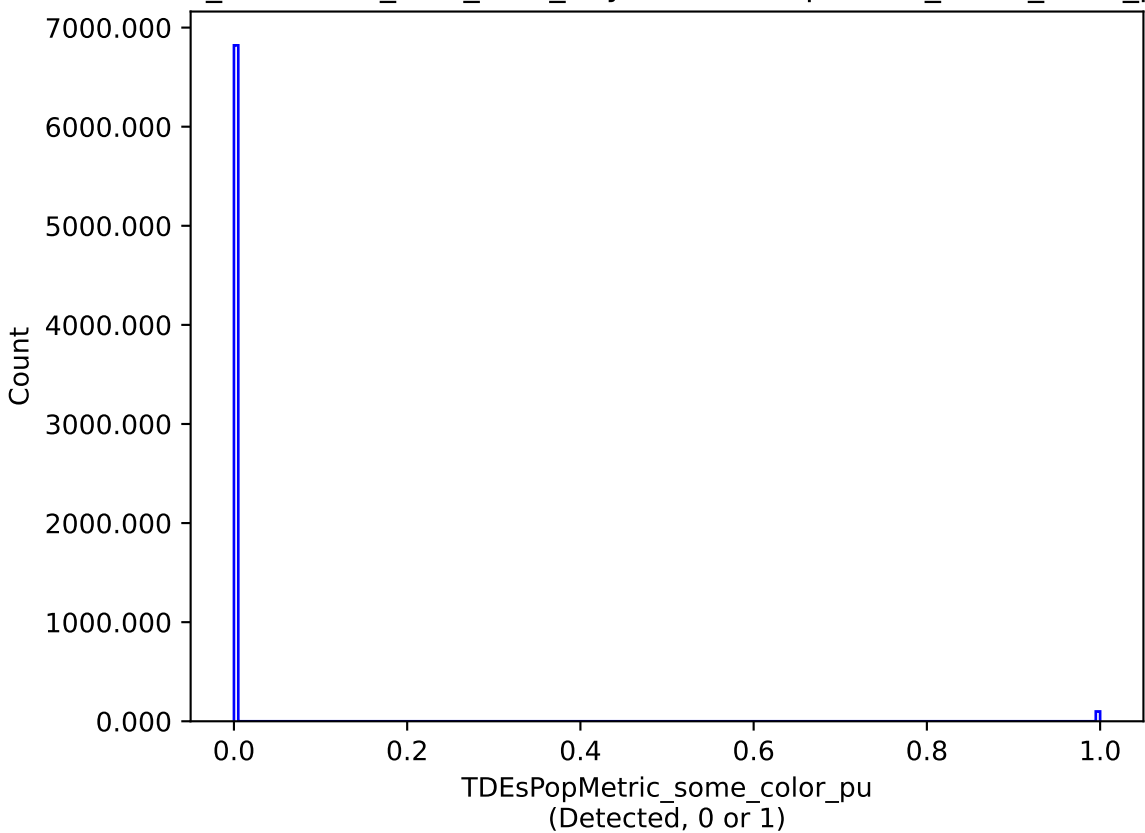
too_combined_s0.8_v3.4_10yrs : TDEsPopMetric_some_color_pu
