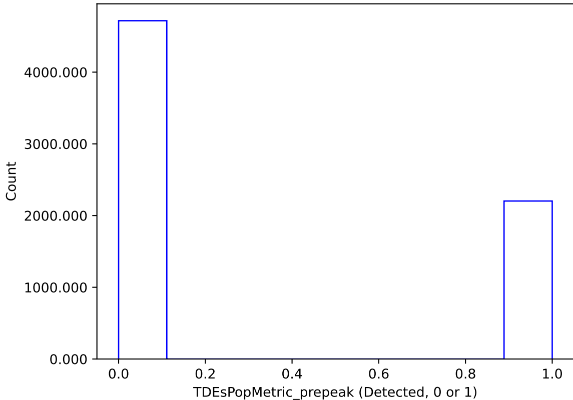
too_combined_s0.8_v3.4_10yrs : TDEsPopMetric_prepeak
