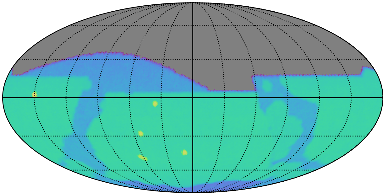
too_combined_s0.8_v3.4_10yrs z: SurfaceBrightLimit
