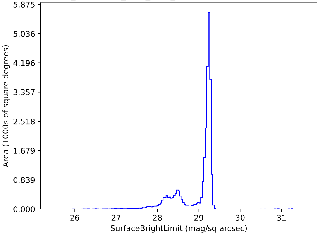
too_combined_s0.8_v3.4_10yrs z: SurfaceBrightLimit
